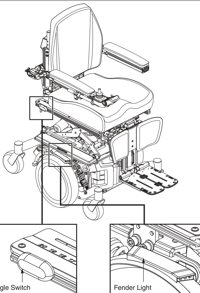
Figure 4. Q6 Edge 2.0 Series with Single Switch to Operate Fender Lights
